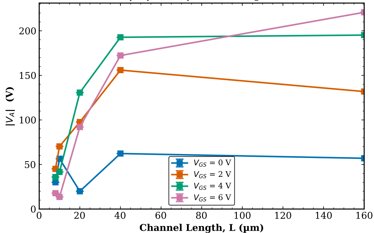
TFT1 Transistor 1 |V_A| vs L | W = 100\text{ }\mu\text{m}
